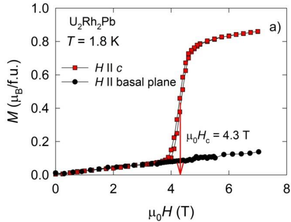
Figure 4.2 Magnetization isotherms of \text{U}_2\text{Rh}_2\text{Pb} measured at T = 1.8 K with the magnetic field parallel to the c -axis and parallel to the randomly oriented basal planes.
