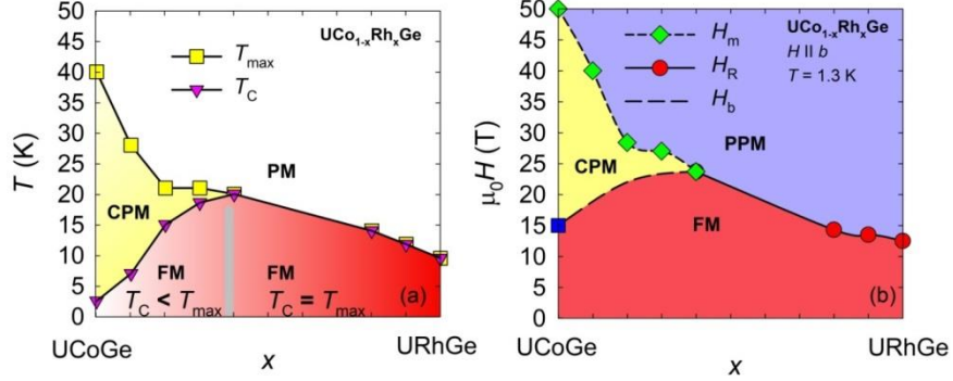
Figure 2.7 a) T - x and b) H - x phase diagrams of the \text{UCo}_{1-x}\text{Rh}_x\text{Ge} system. The value of T_{\text{max}} , H_{\text{R}} , and H_{\text{m}} for URhGe and UCoGe, respectively, were taken from Ref. 78 . The blue point in panel (b) marks the critical field of the ferromagnetic phase boundary in UCoGe; the point was taken from Ref. 86 . The long-dashed line in the H - x diagram tentatively indicates the evolution of FM \rightarrow CPM crossover at H_{\text{b}} . The grey line in the T - x diagrams in panel (a) tentatively separates the low- and high- S_{\text{mag}} concentration regions.
